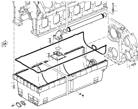
OIL PAN UPC.06E00 0905
