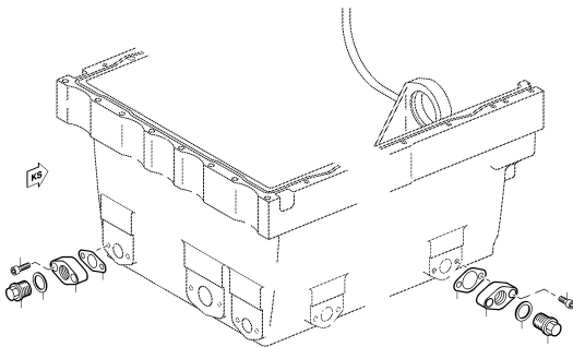
OIL FILLING UPC.06E02 0004
